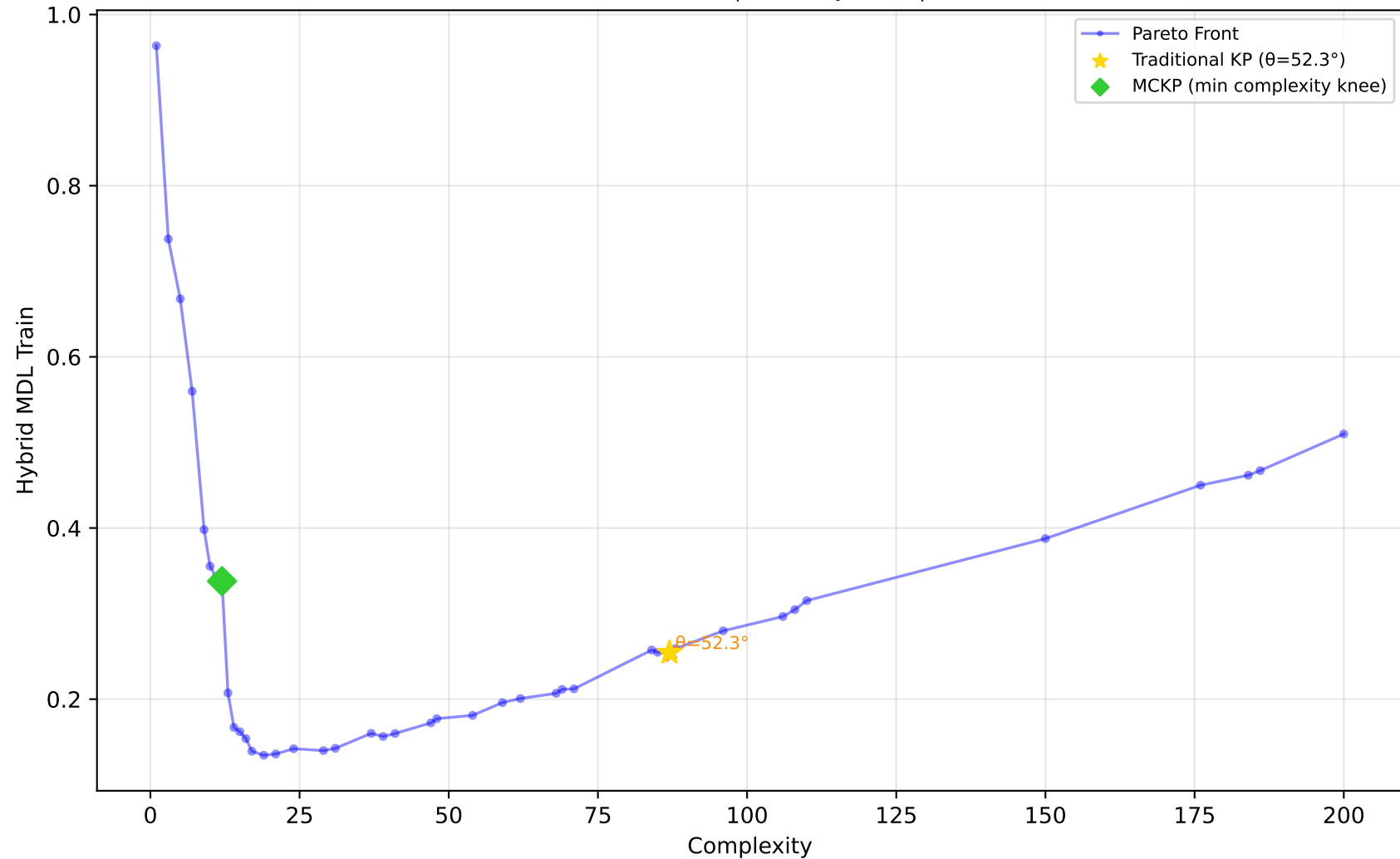
529_pollen - Run 21 - SVP - Hybrid MDL Train \lambda_1=0.60, \lambda_2=0.40, \lambda_3=1.00 | Difficulty: 1.00 | Method: hmr
