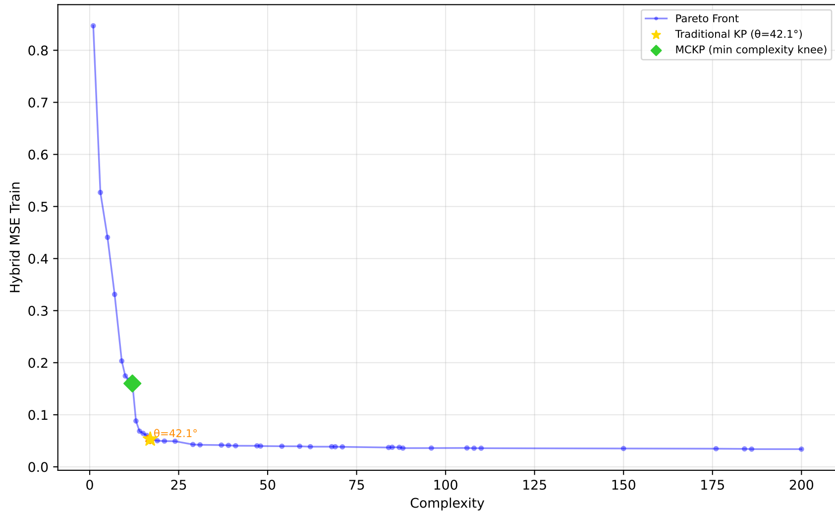
529_pollen - Run 21 - SVP - Hybrid MSE Train \lambda_1=0.10, \lambda_2=0.80, \lambda_3=0.30 | Difficulty: 1.00 | Method: hmr
