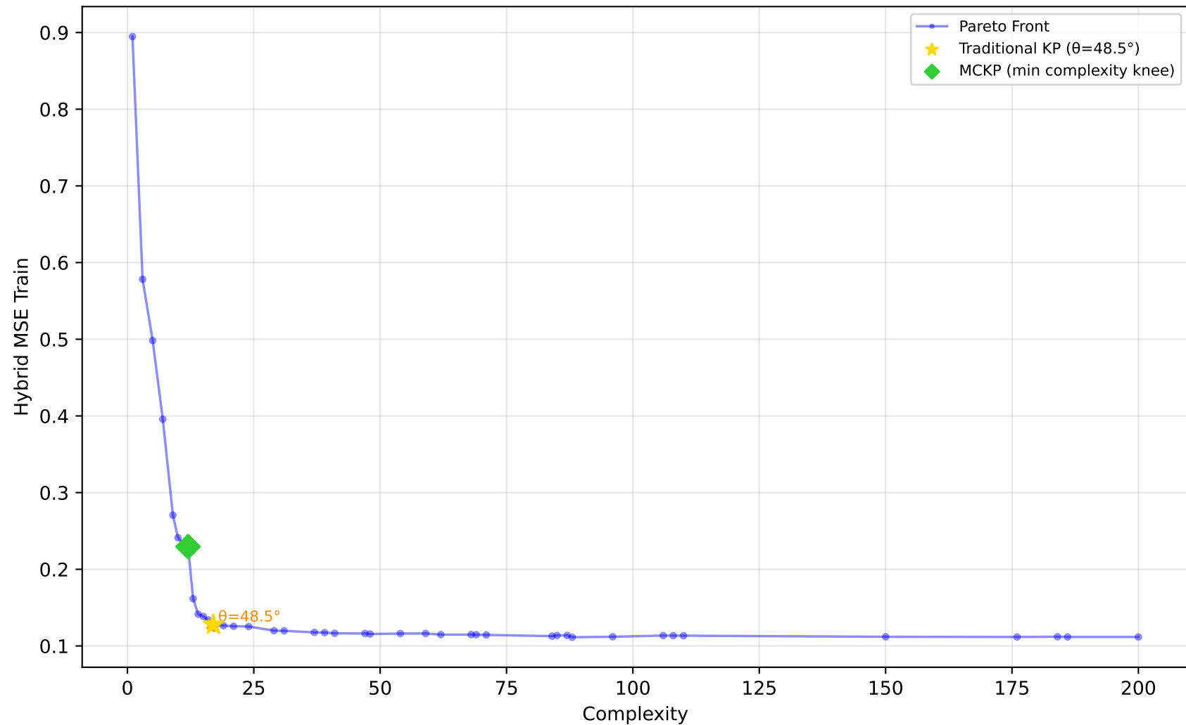
529_pollen - Run 21 - SVP - Hybrid MSE Train \lambda_1=0.60, \lambda_2=0.40, \lambda_3=1.00 | Difficulty: 1.00 | Method: hmr
