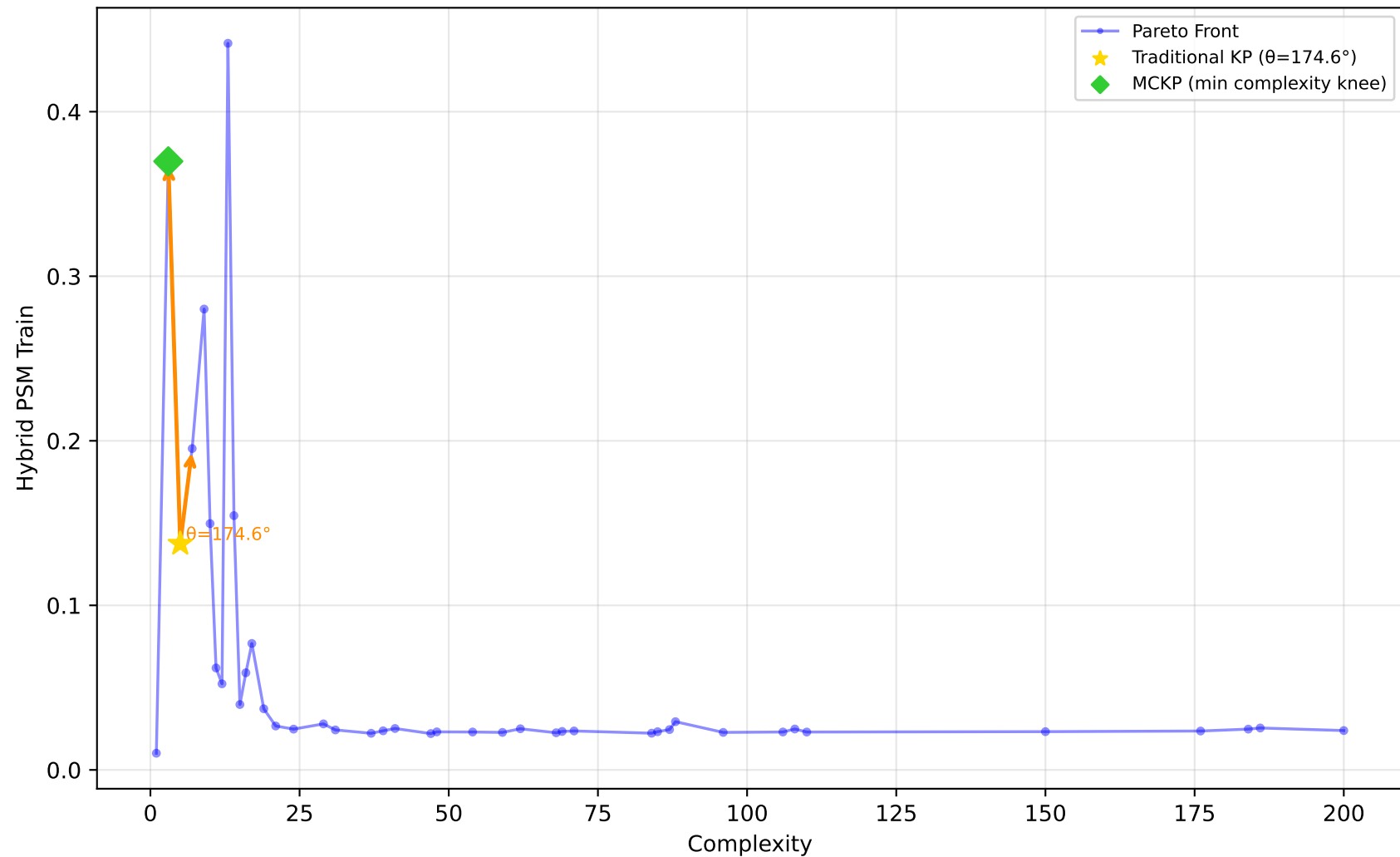
529_pollen - Run 21 - SVP - Hybrid PSM Train \lambda_1=0.10, \lambda_2=0.80, \lambda_3=0.30 | Difficulty: 1.00 | Method: hmr
