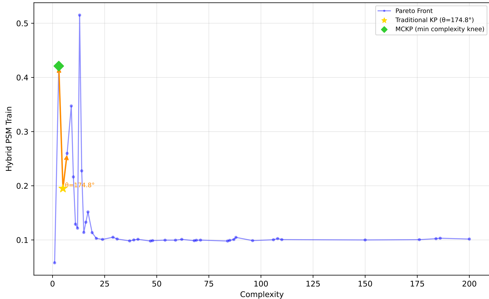
529_pollen - Run 21 - SVP - Hybrid PSM Train \lambda_1=0.60, \lambda_2=0.40, \lambda_3=1.00 | Difficulty: 1.00 | Method: hmr
