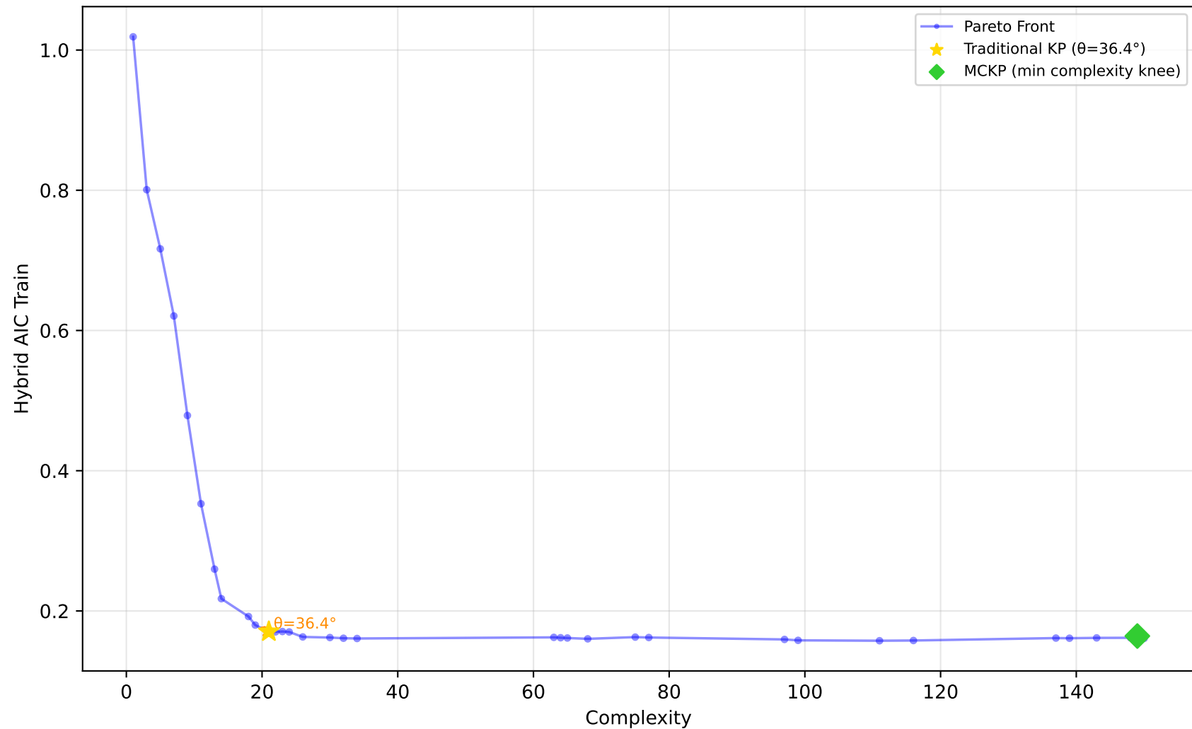
529_pollen - Run 22 - MVP - Hybrid AIC Train \lambda_1=0.90, \lambda_2=0.00, \lambda_3=0.00 | Difficulty: 1.00 | Method: hmr
