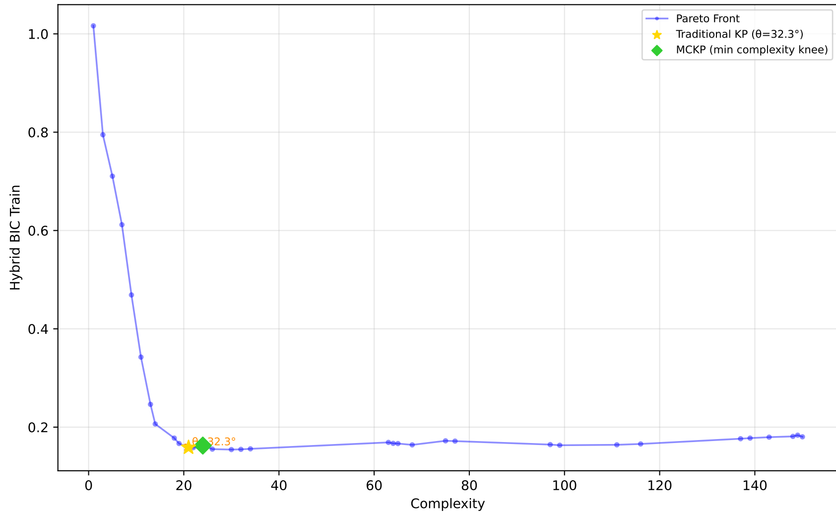
529_pollen - Run 22 - MVP - Hybrid BIC Train \lambda_1=0.90, \lambda_2=0.00, \lambda_3=0.00 | Difficulty: 1.00 | Method: hmr
