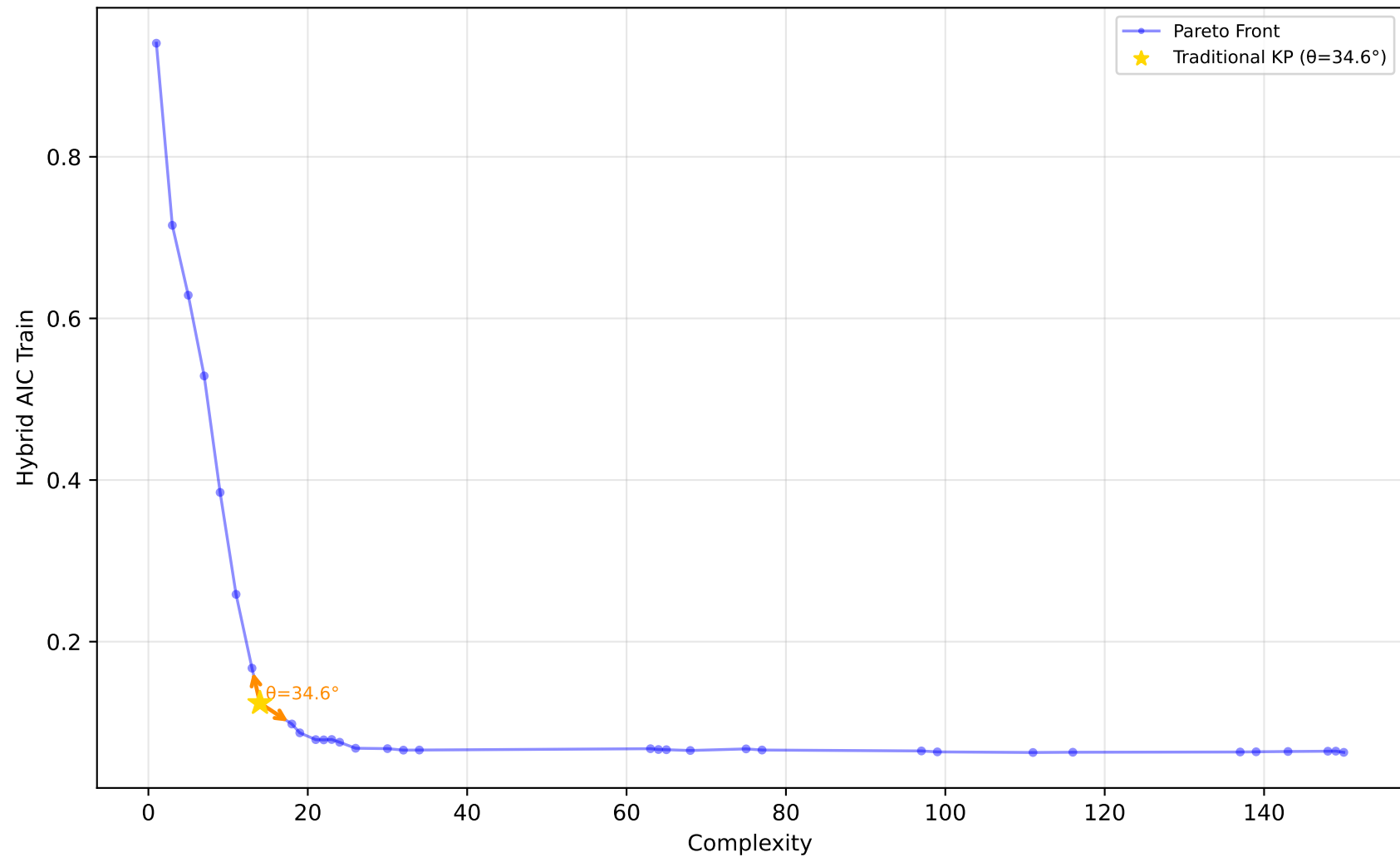
529_pollen - Run 22 - SVP - Hybrid AIC Train \lambda_1=0.10, \lambda_2=0.80, \lambda_3=0.30 | Difficulty: 1.00 | Method: hmr
