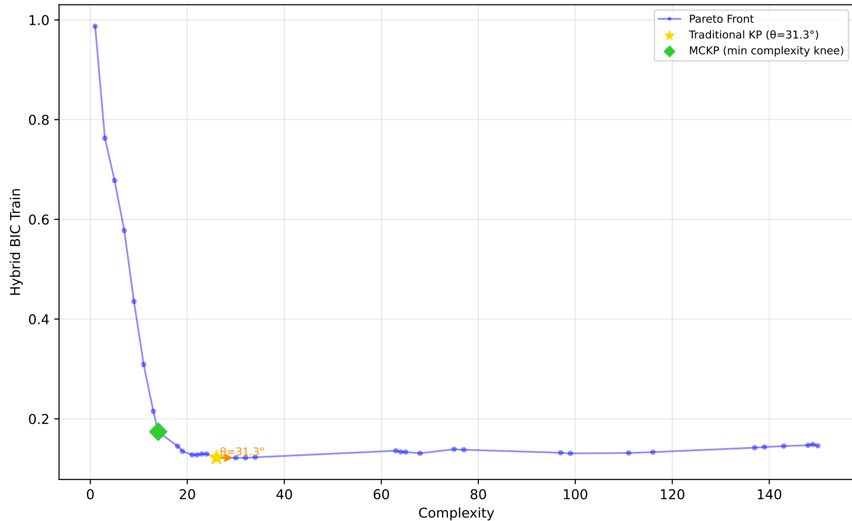
529_pollen - Run 22 - SVP - Hybrid BIC Train \lambda_1=0.60, \lambda_2=0.40, \lambda_3=1.00 | Difficulty: 1.00 | Method: hmr
