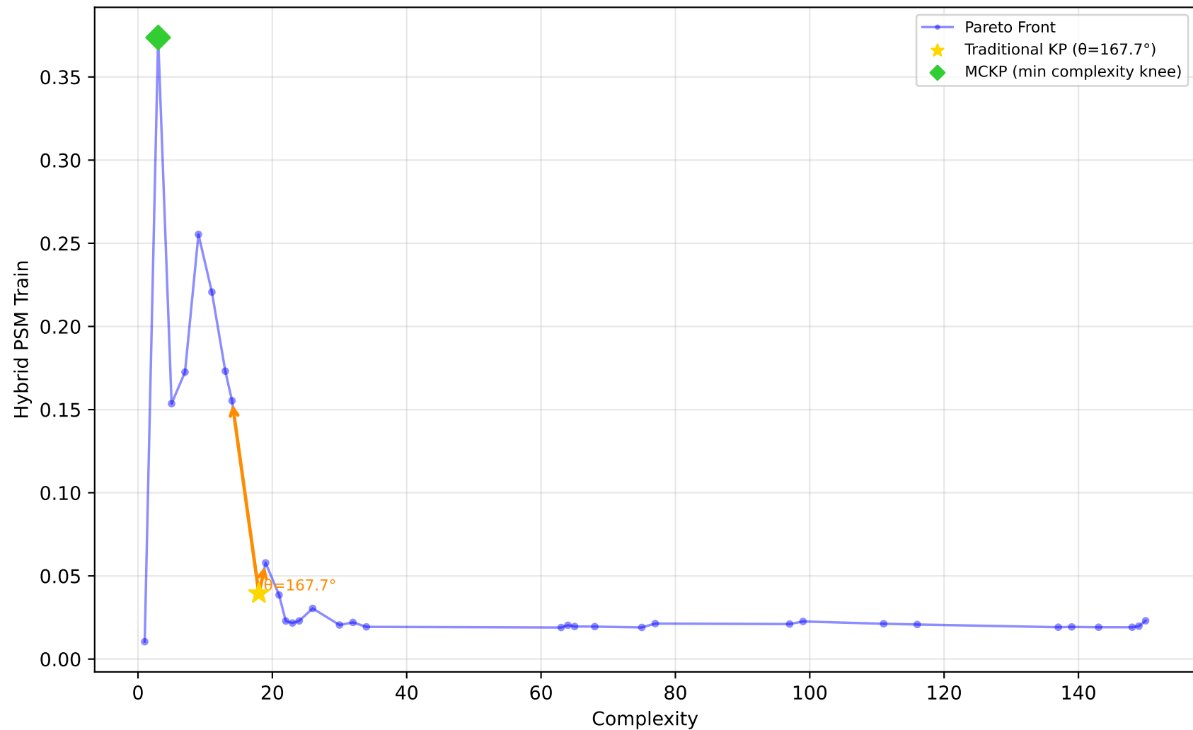
529_pollen - Run 22 - SVP - Hybrid PSM Train \lambda_1=0.10, \lambda_2=0.80, \lambda_3=0.30 | Difficulty: 1.00 | Method: hmr
