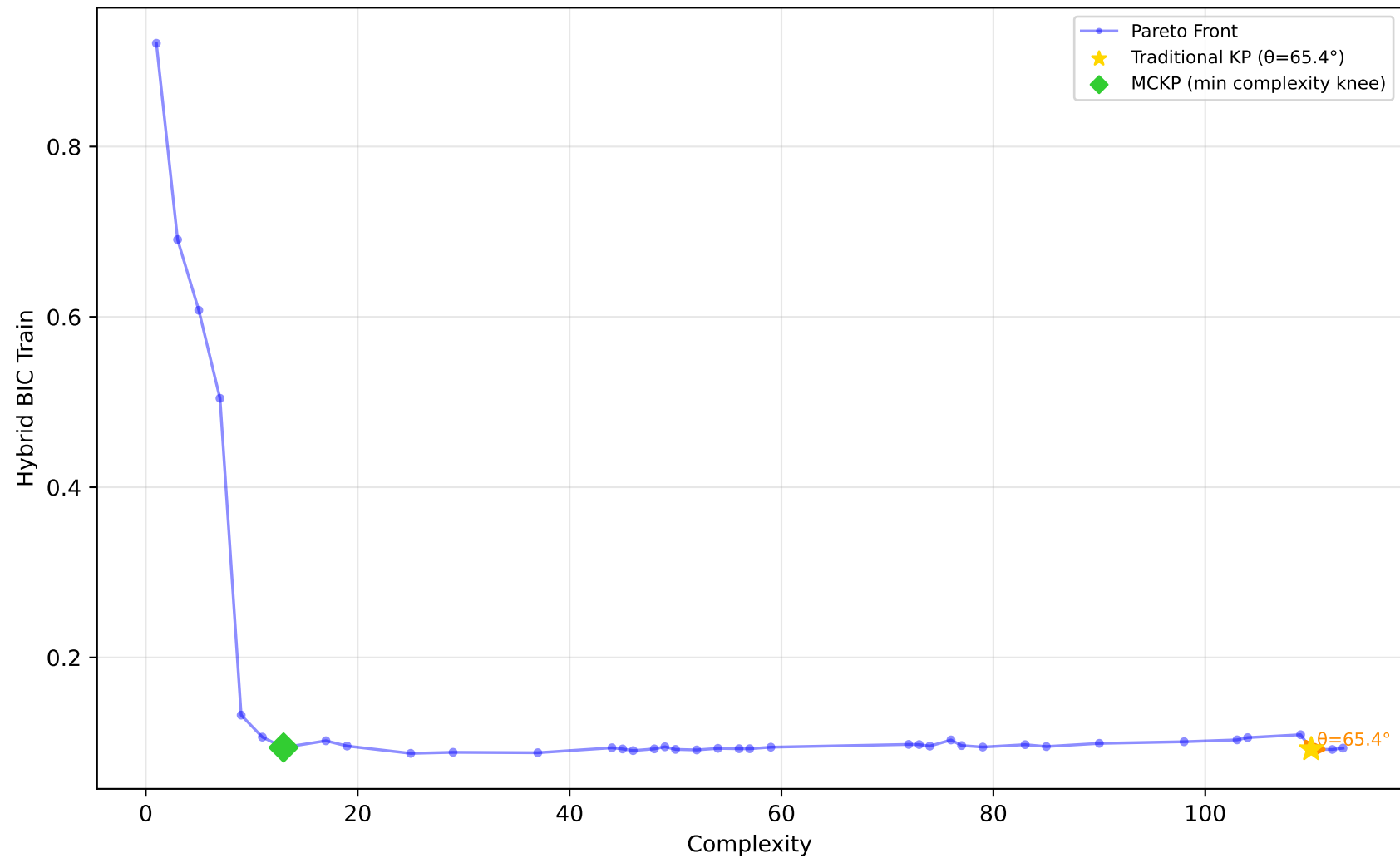
529_pollen - Run 23 - MVP - Hybrid BIC Train \lambda_1=0.00, \lambda_2=1.00, \lambda_3=0.80 | Difficulty: 1.00 | Method: hmr
