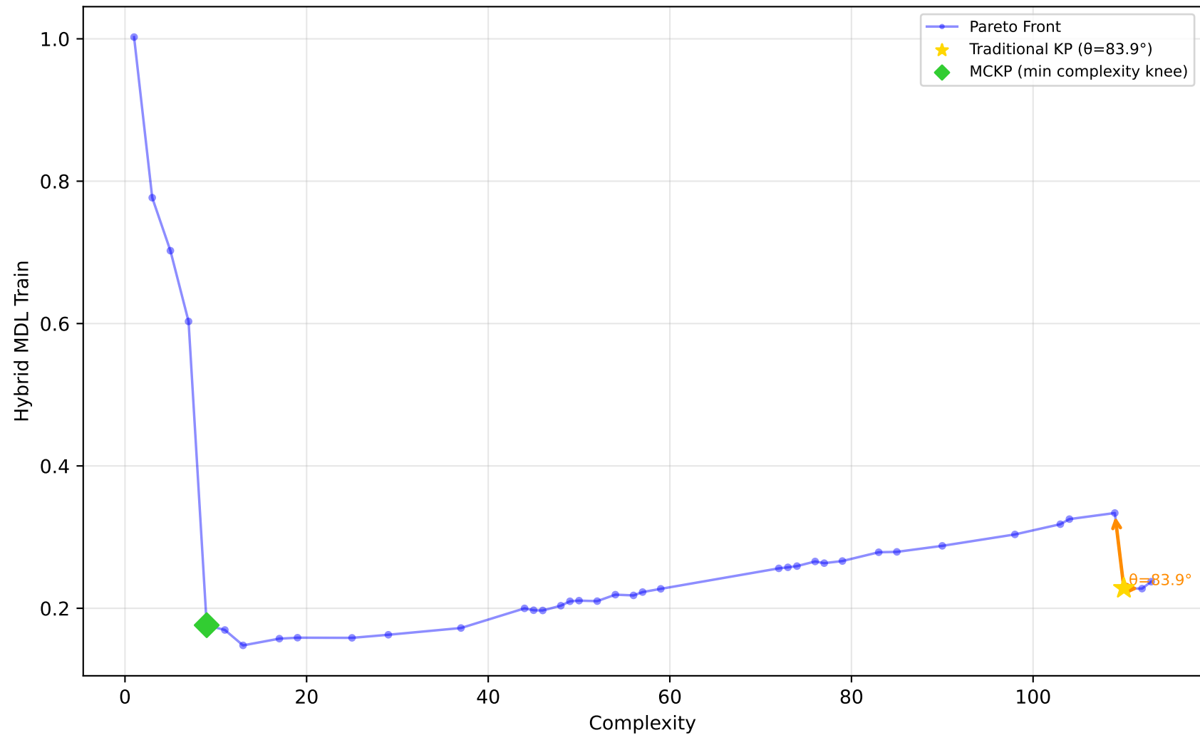
529_pollen - Run 23 - MVP - Hybrid MDL Train \lambda_1=0.90, \lambda_2=0.00, \lambda_3=0.00 | Difficulty: 1.00 | Method: hmr
