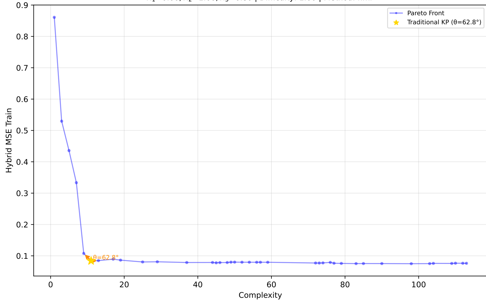
529_pollen - Run 23 - MVP - Hybrid MSE Train \lambda_1=0.00, \lambda_2=1.00, \lambda_3=0.80 | Difficulty: 1.00 | Method: hmr
