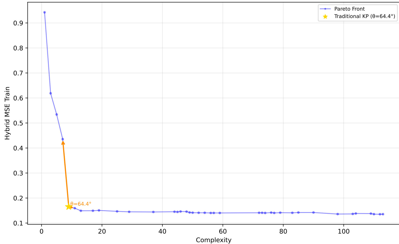
529_pollen - Run 23 - MVP - Hybrid MSE Train \lambda_1=0.90, \lambda_2=0.00, \lambda_3=0.00 | Difficulty: 1.00 | Method: hmr
