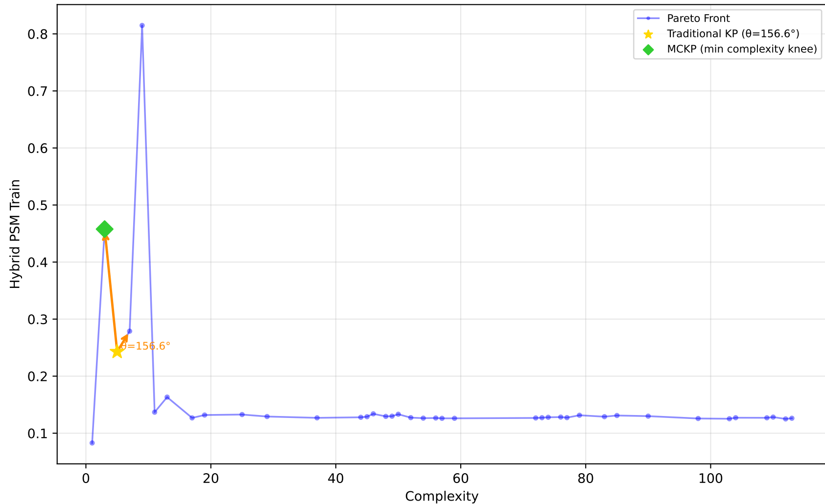
529_pollen - Run 23 - MVP - Hybrid PSM Train \lambda_1=0.90, \lambda_2=0.00, \lambda_3=0.00 | Difficulty: 1.00 | Method: hmr
