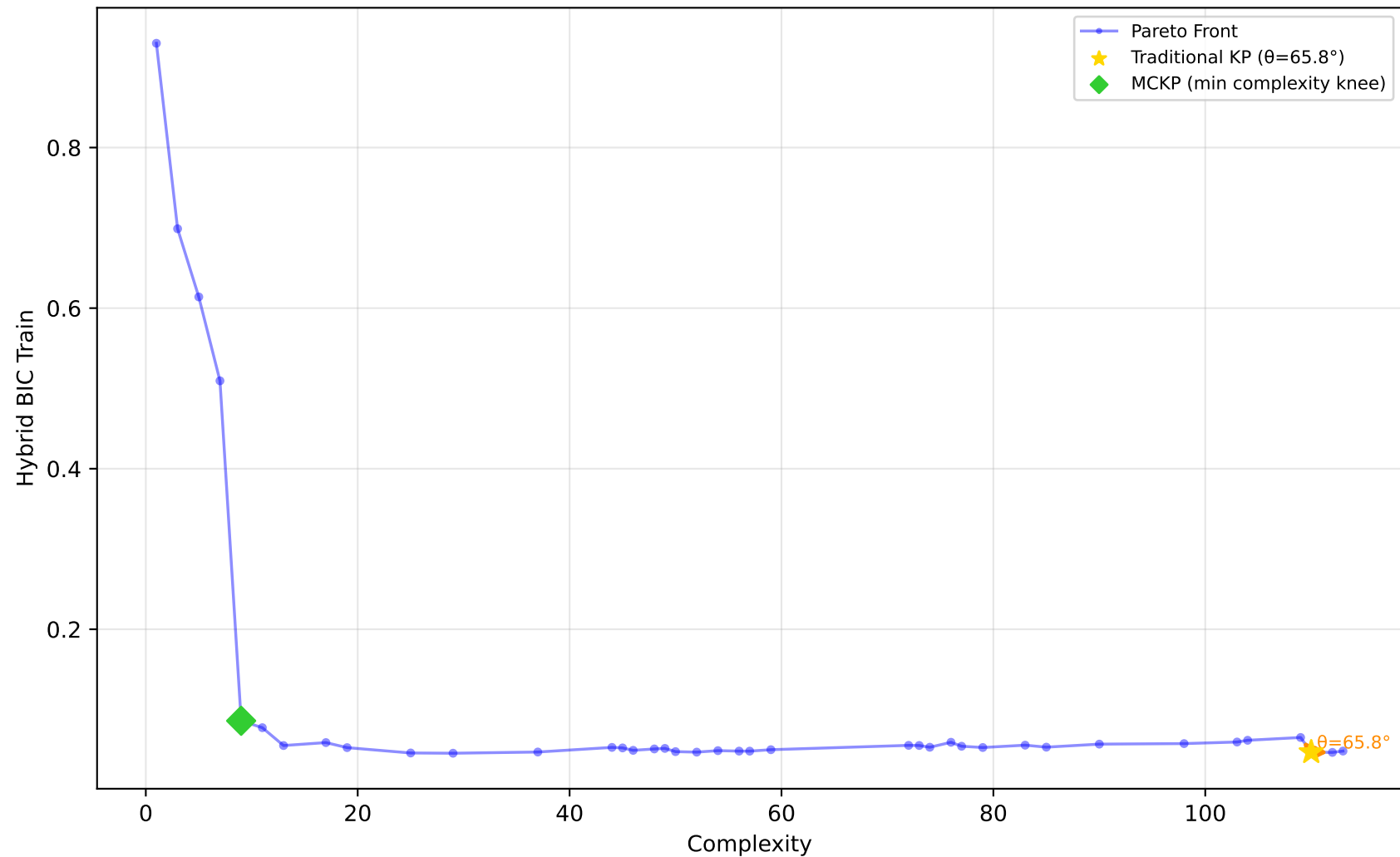
529_pollen - Run 23 - SVP - Hybrid BIC Train \lambda_1=0.10, \lambda_2=0.80, \lambda_3=0.30 | Difficulty: 1.00 | Method: hmr
