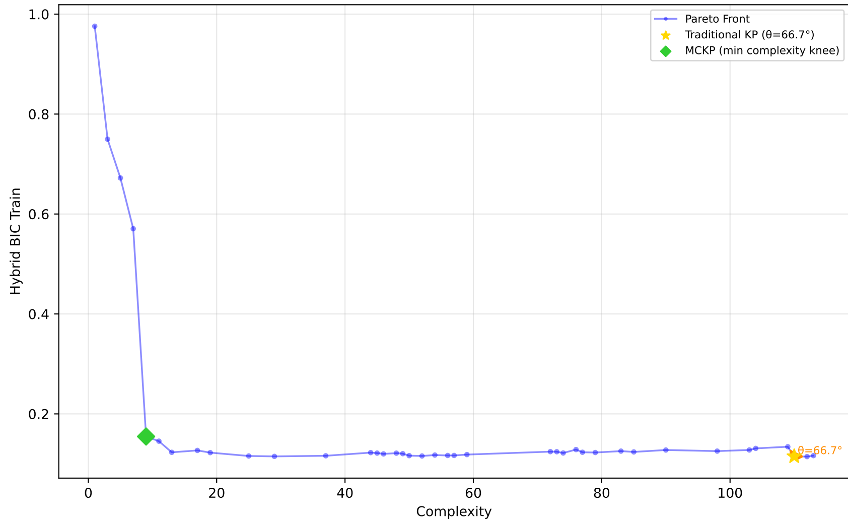
529_pollen - Run 23 - SVP - Hybrid BIC Train \lambda_1=0.60 , \lambda_2=0.40 , \lambda_3=1.00 | Difficulty: 1.00 | Method: hmr
