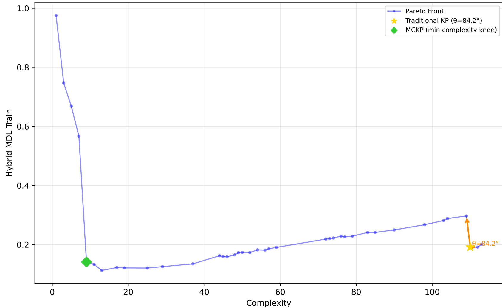
529_pollen - Run 23 - SVP - Hybrid MDL Train \lambda_1=0.60, \lambda_2=0.40, \lambda_3=1.00 | Difficulty: 1.00 | Method: hmr
