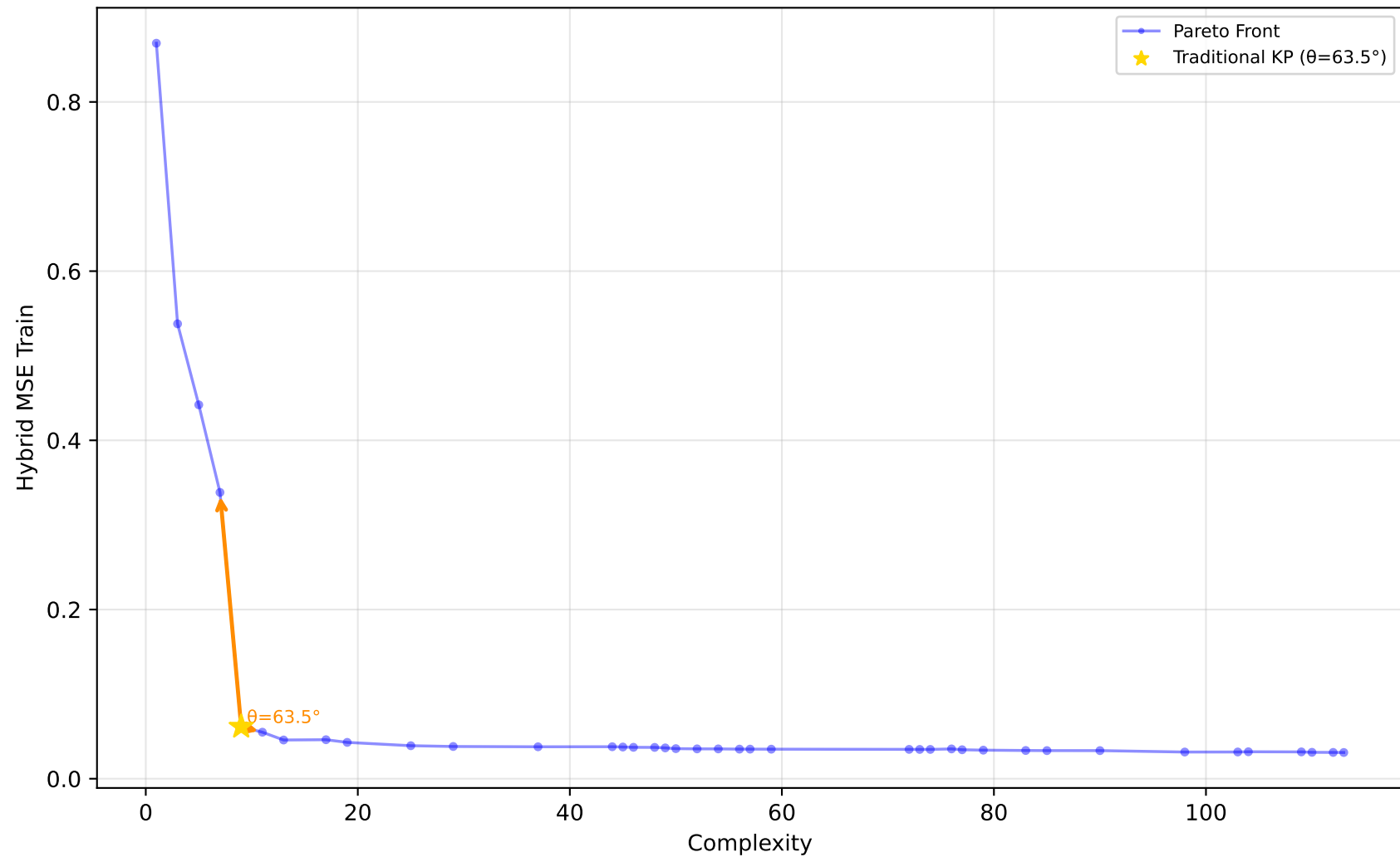
529_pollen - Run 23 - SVP - Hybrid MSE Train \lambda_1=0.10, \lambda_2=0.80, \lambda_3=0.30 | Difficulty: 1.00 | Method: hmr
