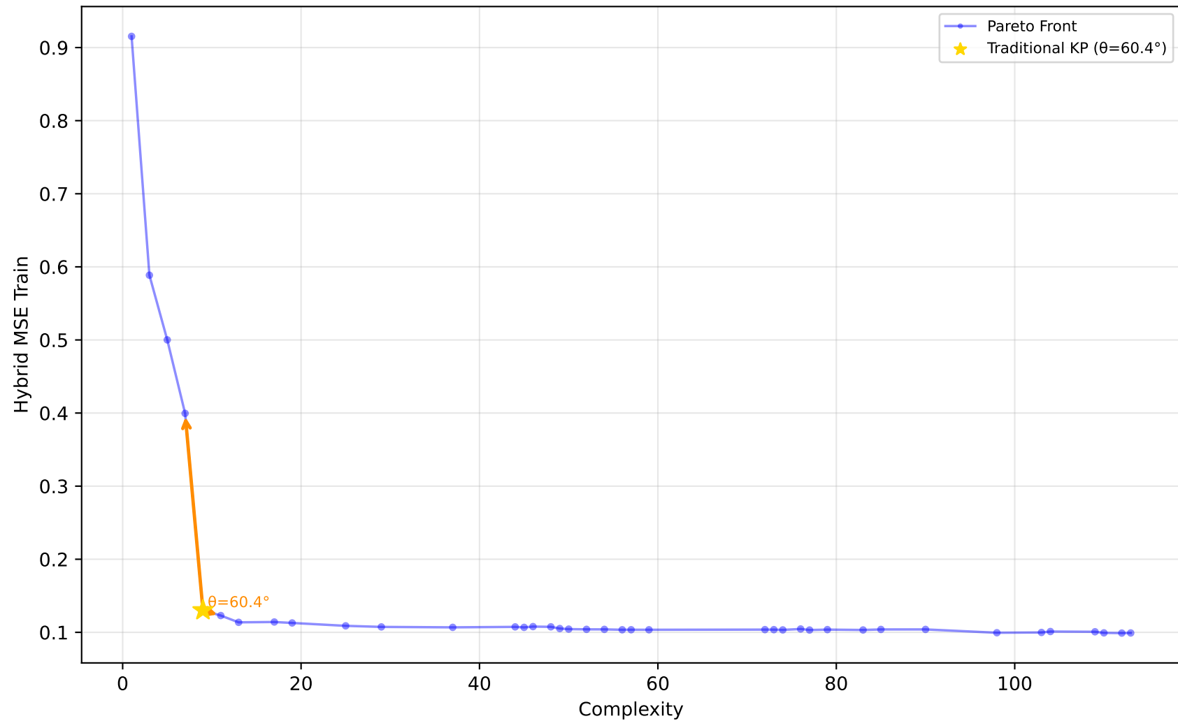
529_pollen - Run 23 - SVP - Hybrid MSE Train \lambda_1=0.60, \lambda_2=0.40, \lambda_3=1.00 | Difficulty: 1.00 | Method: hmr
