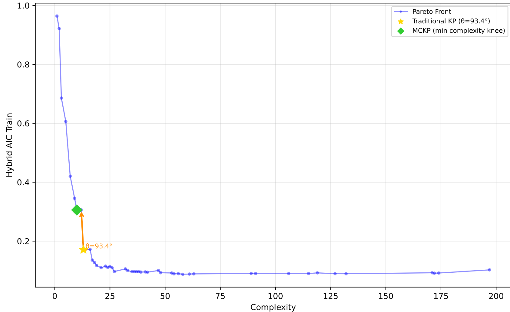
529_pollen - Run 24 - MVP - Hybrid AIC Train \lambda_1=0.00, \lambda_2=1.00, \lambda_3=0.80 | Difficulty: 1.00 | Method: hmr
