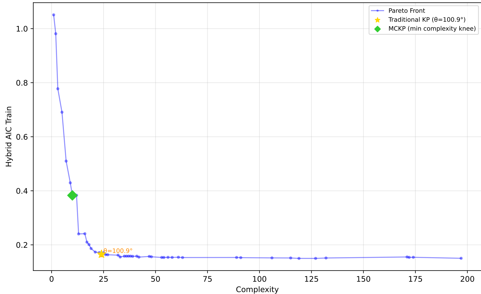
529_pollen - Run 24 - MVP - Hybrid AIC Train \lambda_1=0.90, \lambda_2=0.00, \lambda_3=0.00 | Difficulty: 1.00 | Method: hmr
