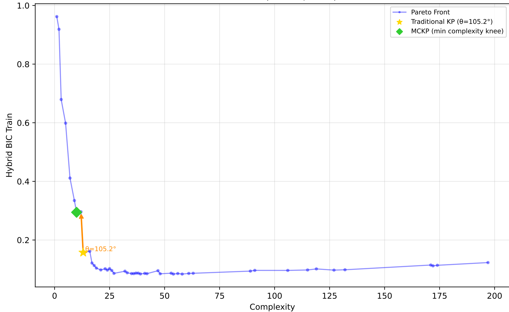
529_pollen - Run 24 - MVP - Hybrid BIC Train \lambda_1=0.00, \lambda_2=1.00, \lambda_3=0.80 | Difficulty: 1.00 | Method: hmr
