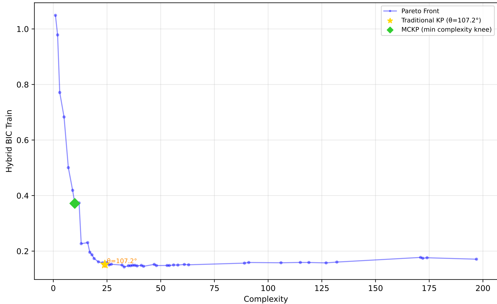
529_pollen - Run 24 - MVP - Hybrid BIC Train \lambda_1=0.90, \lambda_2=0.00, \lambda_3=0.00 | Difficulty: 1.00 | Method: hmr
