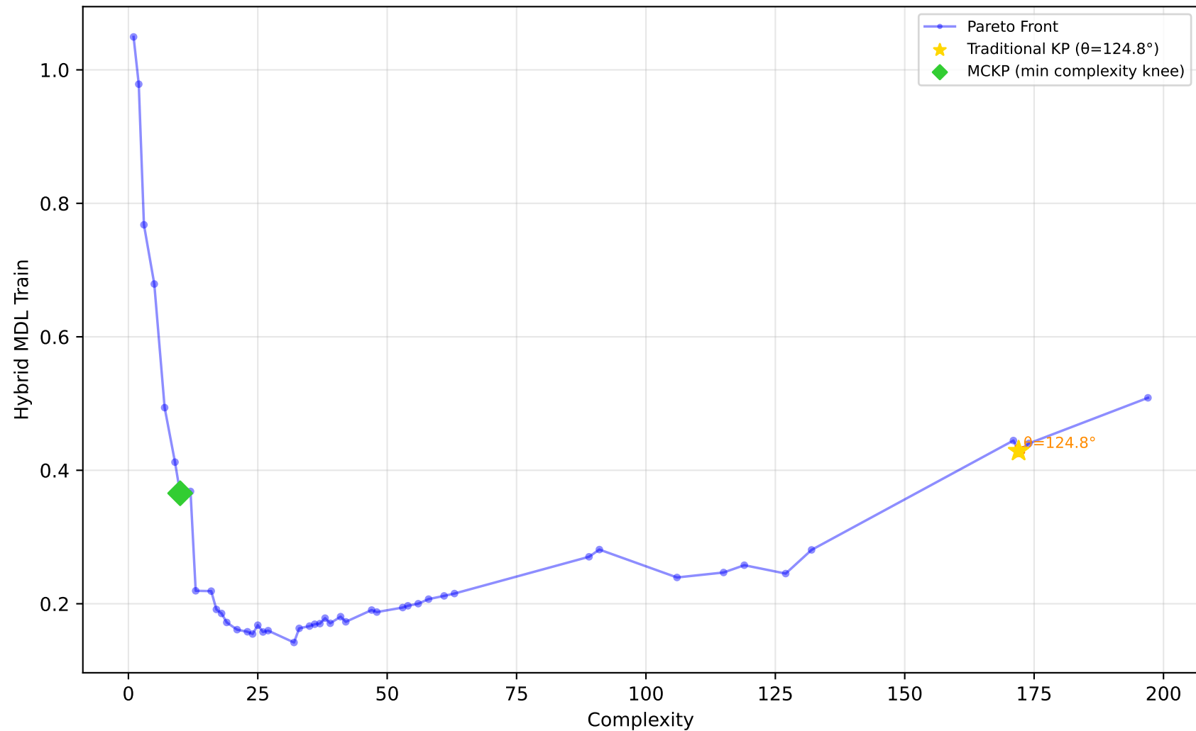
529_pollen - Run 24 - MVP - Hybrid MDL Train \lambda_1=0.90, \lambda_2=0.00, \lambda_3=0.00 | Difficulty: 1.00 | Method: hmr
