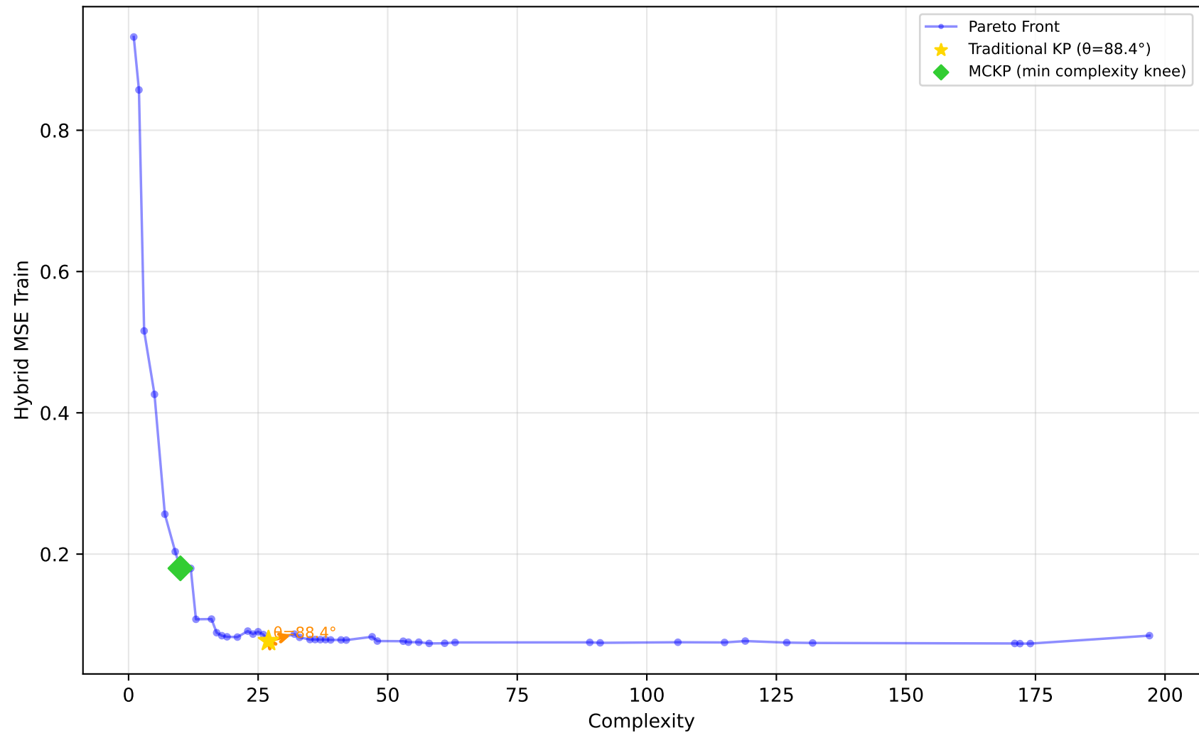
529_pollen - Run 24 - MVP - Hybrid MSE Train \lambda_1=0.00, \lambda_2=1.00, \lambda_3=0.80 | Difficulty: 1.00 | Method: hmr
