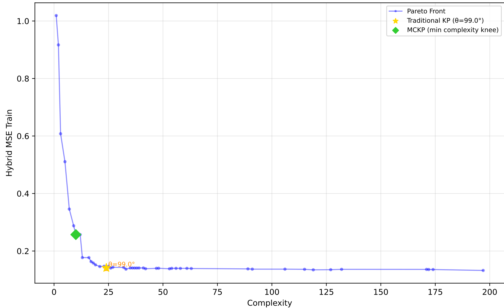
529_pollen - Run 24 - MVP - Hybrid MSE Train \lambda_1=0.90, \lambda_2=0.00, \lambda_3=0.00 | Difficulty: 1.00 | Method: hmr
