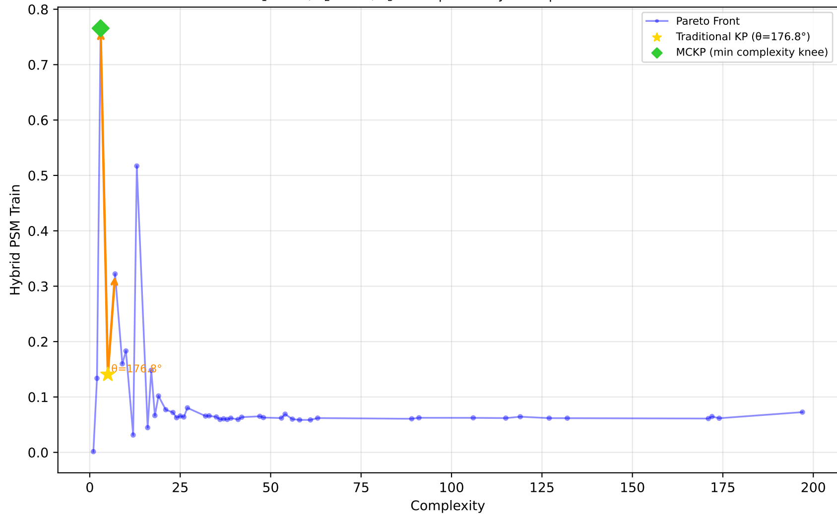
529_pollen - Run 24 - MVP - Hybrid PSM Train \lambda_1=0.00, \lambda_2=1.00, \lambda_3=0.80 | Difficulty: 1.00 | Method: hmr
