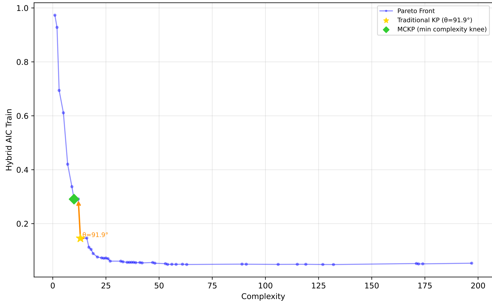
529_pollen - Run 24 - SVP - Hybrid AIC Train \lambda_1=0.10 , \lambda_2=0.80 , \lambda_3=0.30 | Difficulty: 1.00 | Method: hmr
