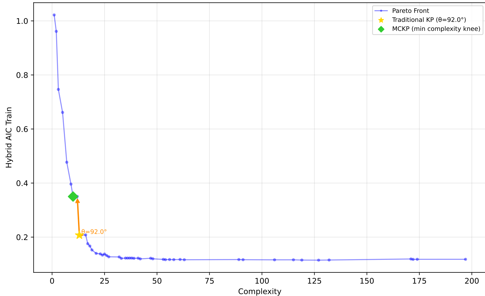
529_pollen - Run 24 - SVP - Hybrid AIC Train \lambda_1=0.60, \lambda_2=0.40, \lambda_3=1.00 | Difficulty: 1.00 | Method: hmr
