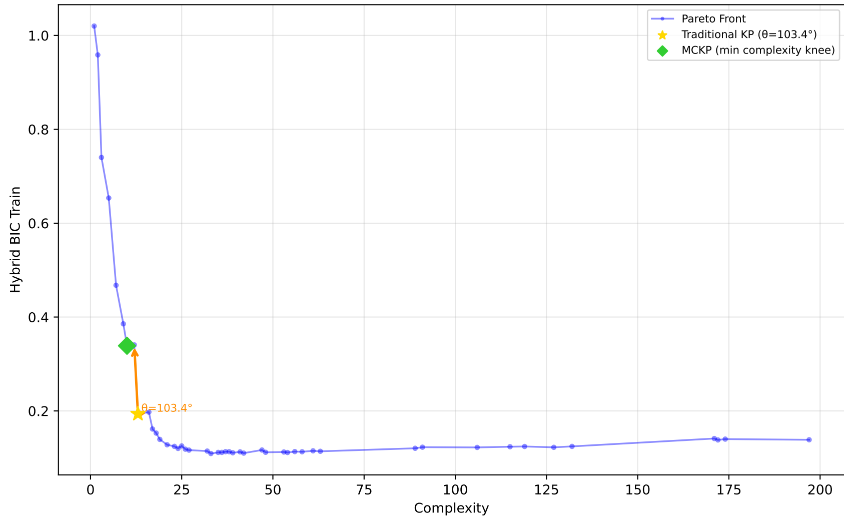
529_pollen - Run 24 - SVP - Hybrid BIC Train \lambda_1=0.60, \lambda_2=0.40, \lambda_3=1.00 | Difficulty: 1.00 | Method: hmr
