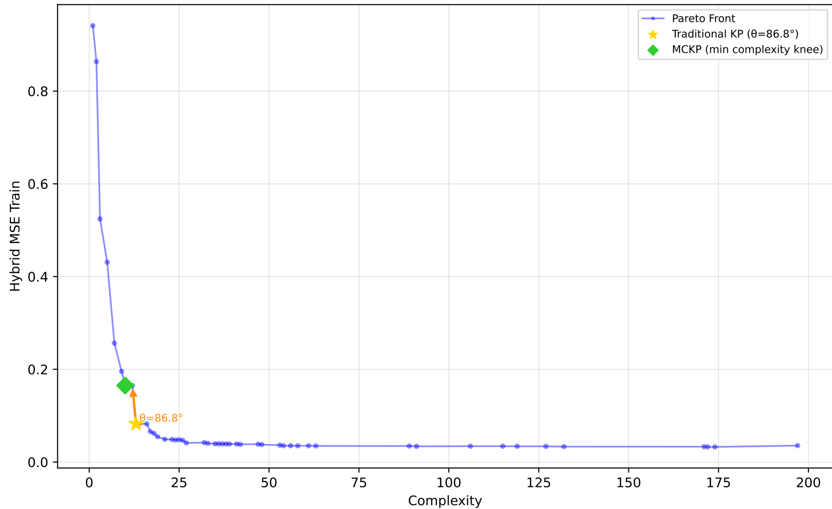
529_pollen - Run 24 - SVP - Hybrid MSE Train \lambda_1=0.10, \lambda_2=0.80, \lambda_3=0.30 | Difficulty: 1.00 | Method: hmr
