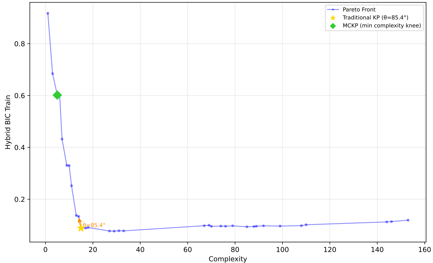
529_pollen - Run 25 - MVP - Hybrid BIC Train \lambda_1=0.00, \lambda_2=1.00, \lambda_3=0.80 | Difficulty: 1.00 | Method: hmr
