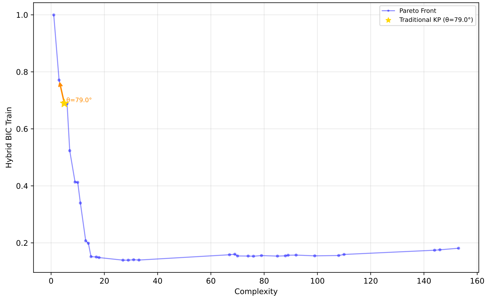
529_pollen - Run 25 - MVP - Hybrid BIC Train \lambda_1=0.90, \lambda_2=0.00, \lambda_3=0.00 | Difficulty: 1.00 | Method: hmr
