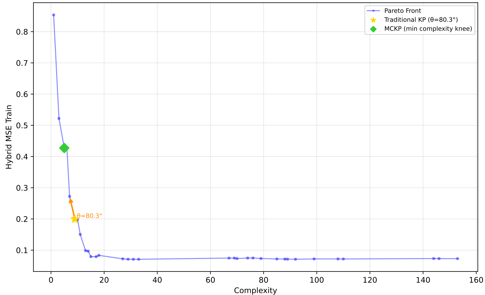
529_pollen - Run 25 - MVP - Hybrid MSE Train \lambda_1=0.00, \lambda_2=1.00, \lambda_3=0.80 | Difficulty: 1.00 | Method: hmr
