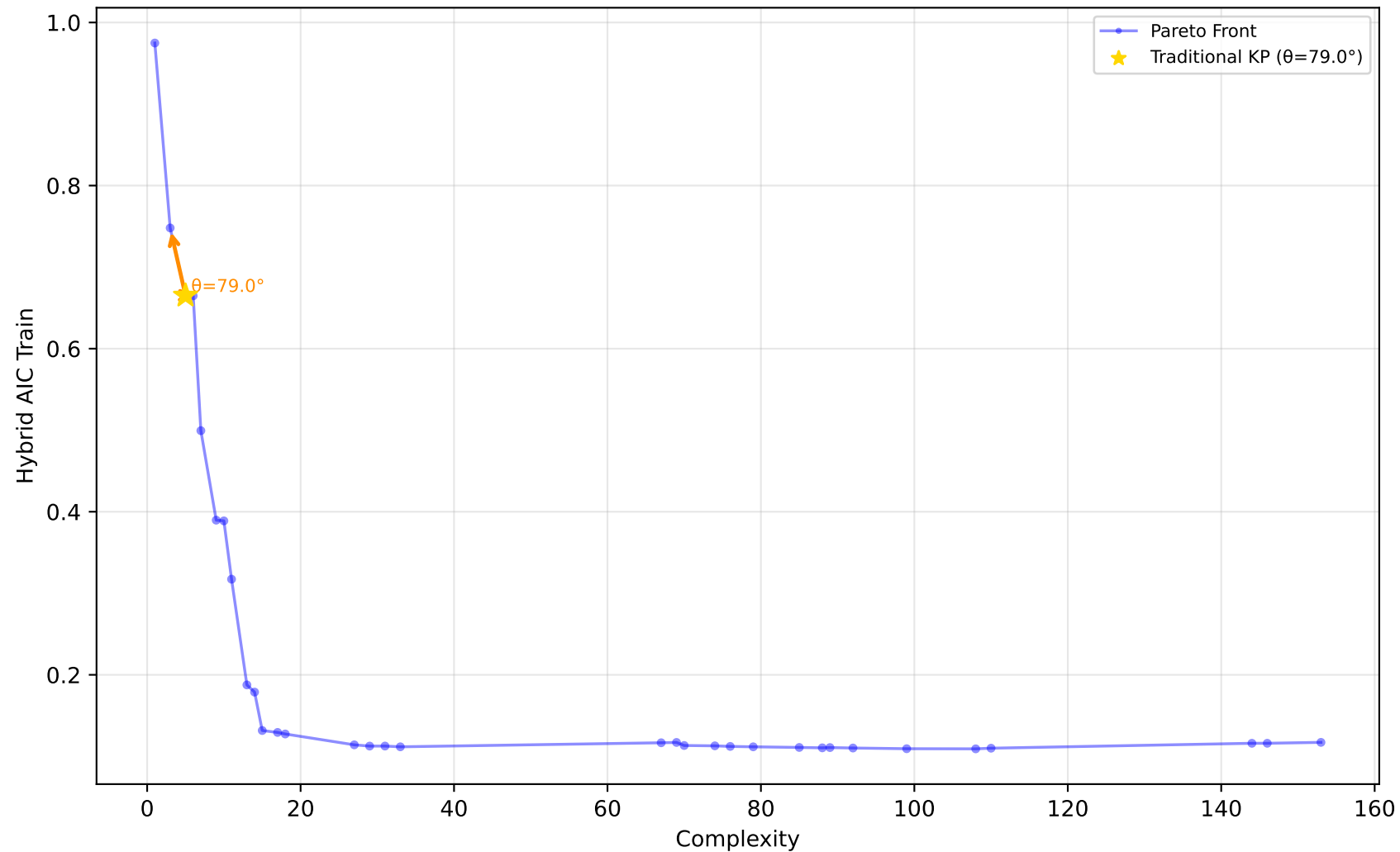
529_pollen - Run 25 - SVP - Hybrid AIC Train \lambda_1=0.60, \lambda_2=0.40, \lambda_3=1.00 | Difficulty: 1.00 | Method: hmr
