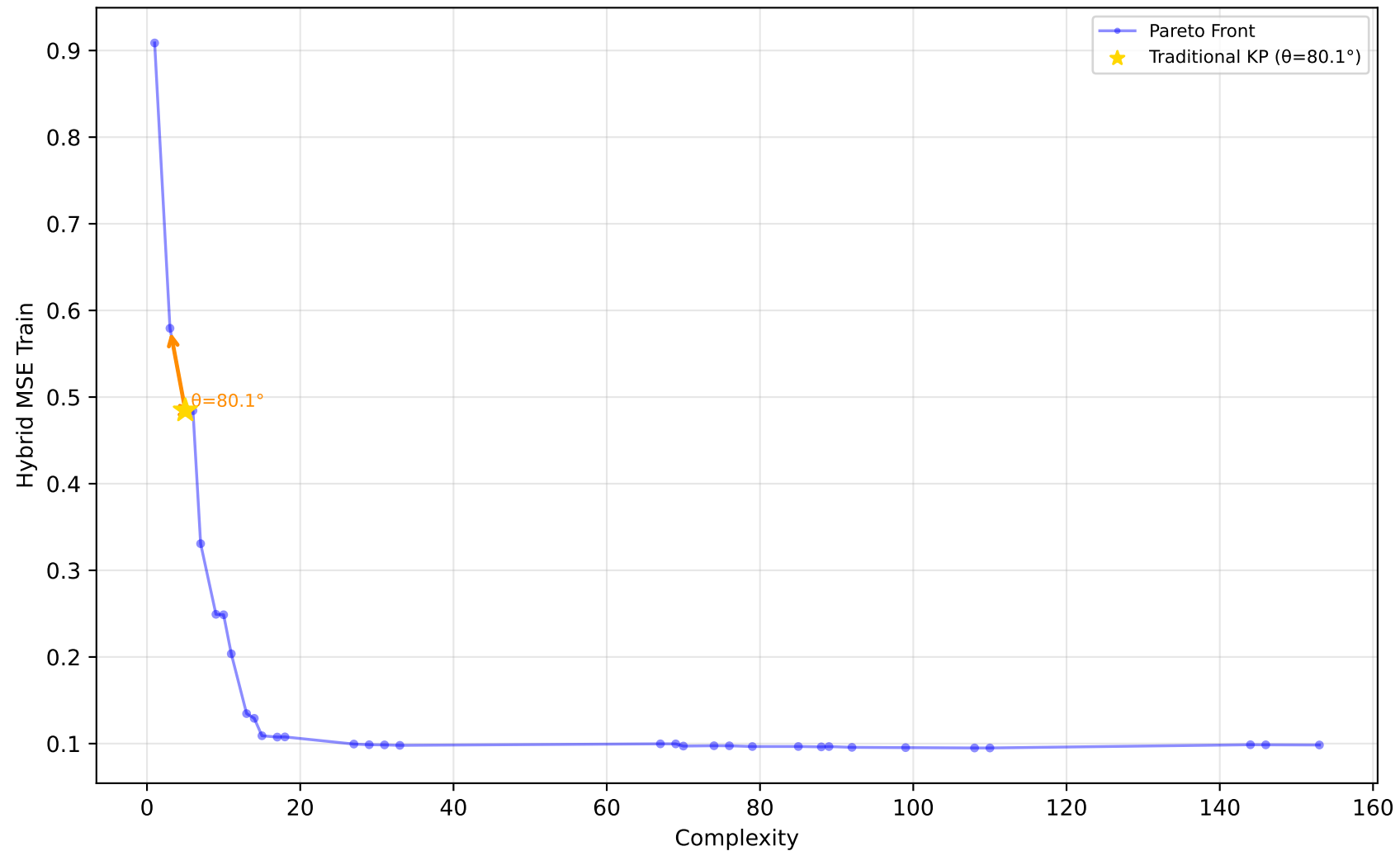
529_pollen - Run 25 - SVP - Hybrid MSE Train \lambda_1=0.60, \lambda_2=0.40, \lambda_3=1.00 | Difficulty: 1.00 | Method: hmr
