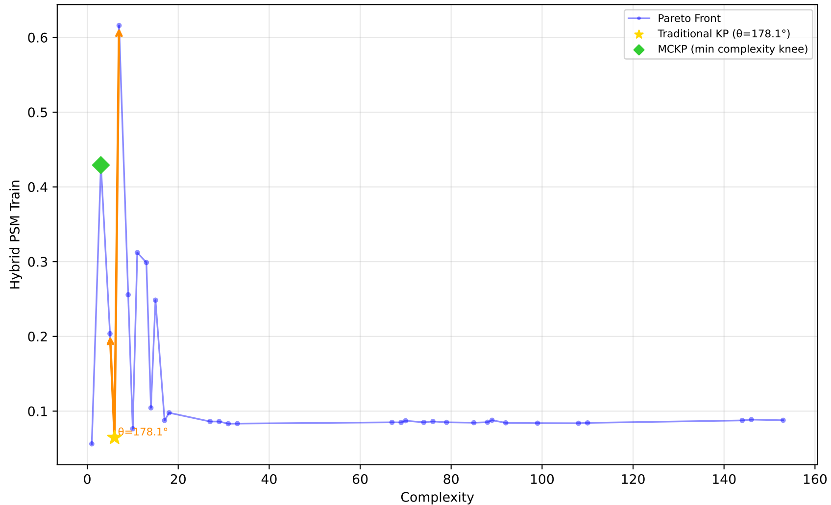
529_pollen - Run 25 - SVP - Hybrid PSM Train \lambda_1=0.60, \lambda_2=0.40, \lambda_3=1.00 | Difficulty: 1.00 | Method: hmr
