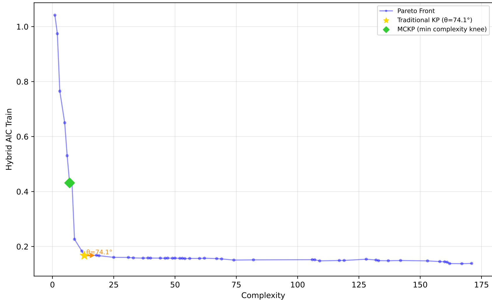
529_pollen - Run 26 - MVP - Hybrid AIC Train \lambda_1=0.90, \lambda_2=0.00, \lambda_3=0.00 | Difficulty: 1.00 | Method: hmr
