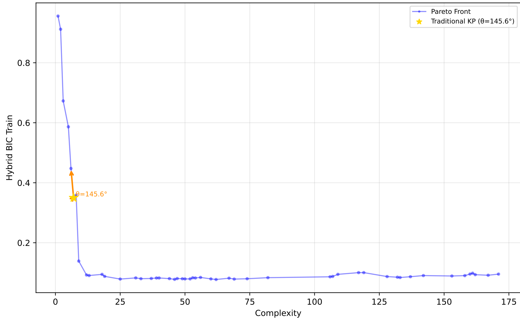
529_pollen - Run 26 - MVP - Hybrid BIC Train \lambda_1=0.00, \lambda_2=1.00, \lambda_3=0.80 | Difficulty: 1.00 | Method: hmr
