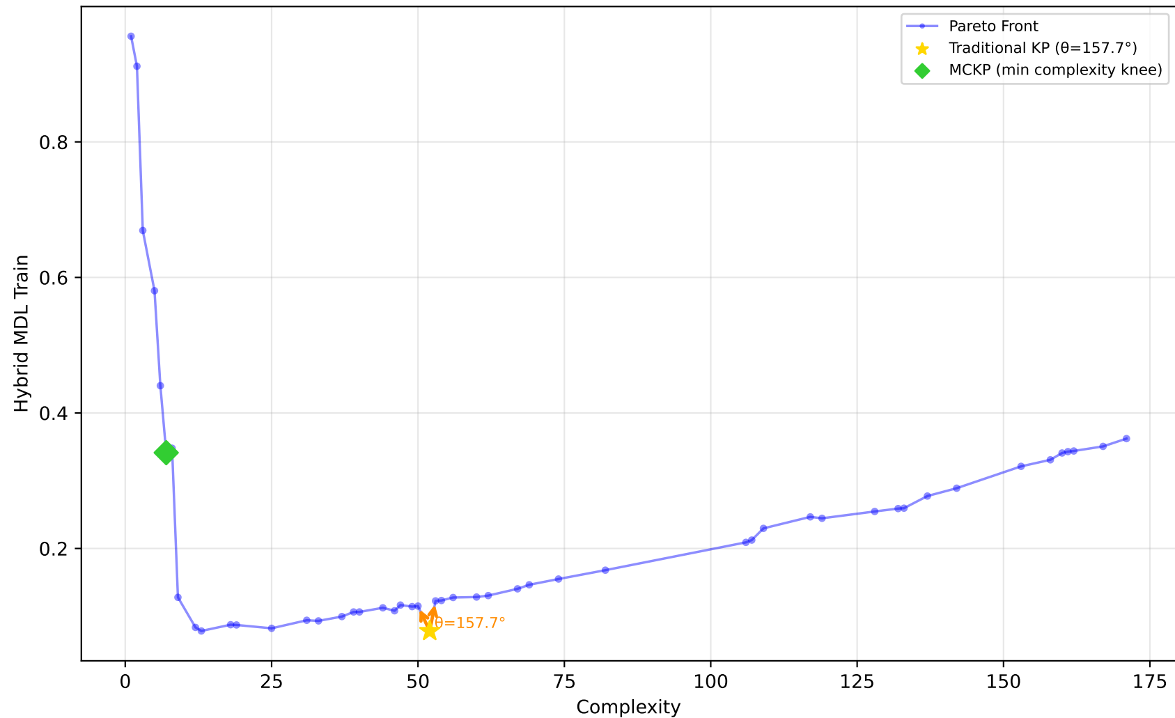
529_pollen - Run 26 - MVP - Hybrid MDL Train \lambda_1=0.00, \lambda_2=1.00, \lambda_3=0.80 | Difficulty: 1.00 | Method: hmr
