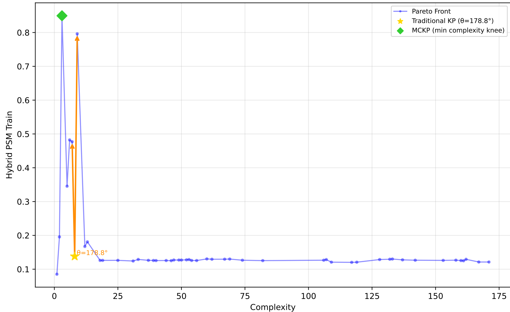
529_pollen - Run 26 - MVP - Hybrid PSM Train \lambda_1=0.90, \lambda_2=0.00, \lambda_3=0.00 | Difficulty: 1.00 | Method: hmr
