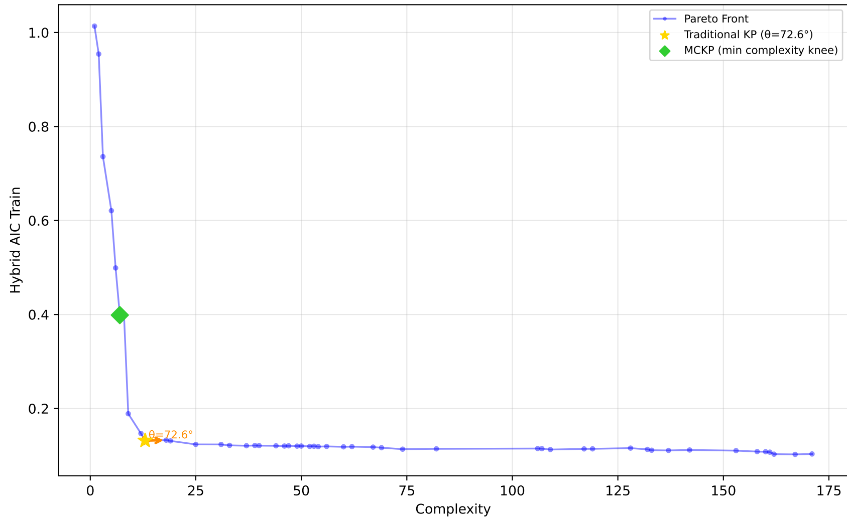
529_pollen - Run 26 - SVP - Hybrid AIC Train \lambda_1=0.60, \lambda_2=0.40, \lambda_3=1.00 | Difficulty: 1.00 | Method: hmr
