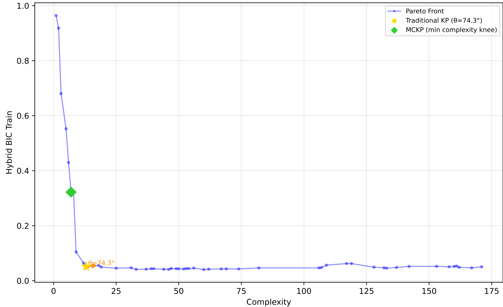
529_pollen - Run 26 - SVP - Hybrid BIC Train \lambda_1=0.10, \lambda_2=0.80, \lambda_3=0.30 | Difficulty: 1.00 | Method: hmr
