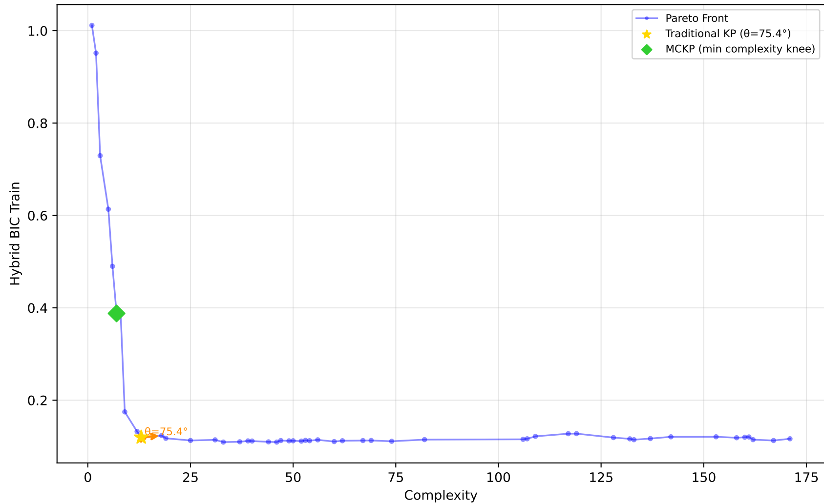
529_pollen - Run 26 - SVP - Hybrid BIC Train \lambda_1=0.60, \lambda_2=0.40, \lambda_3=1.00 | Difficulty: 1.00 | Method: hmr
