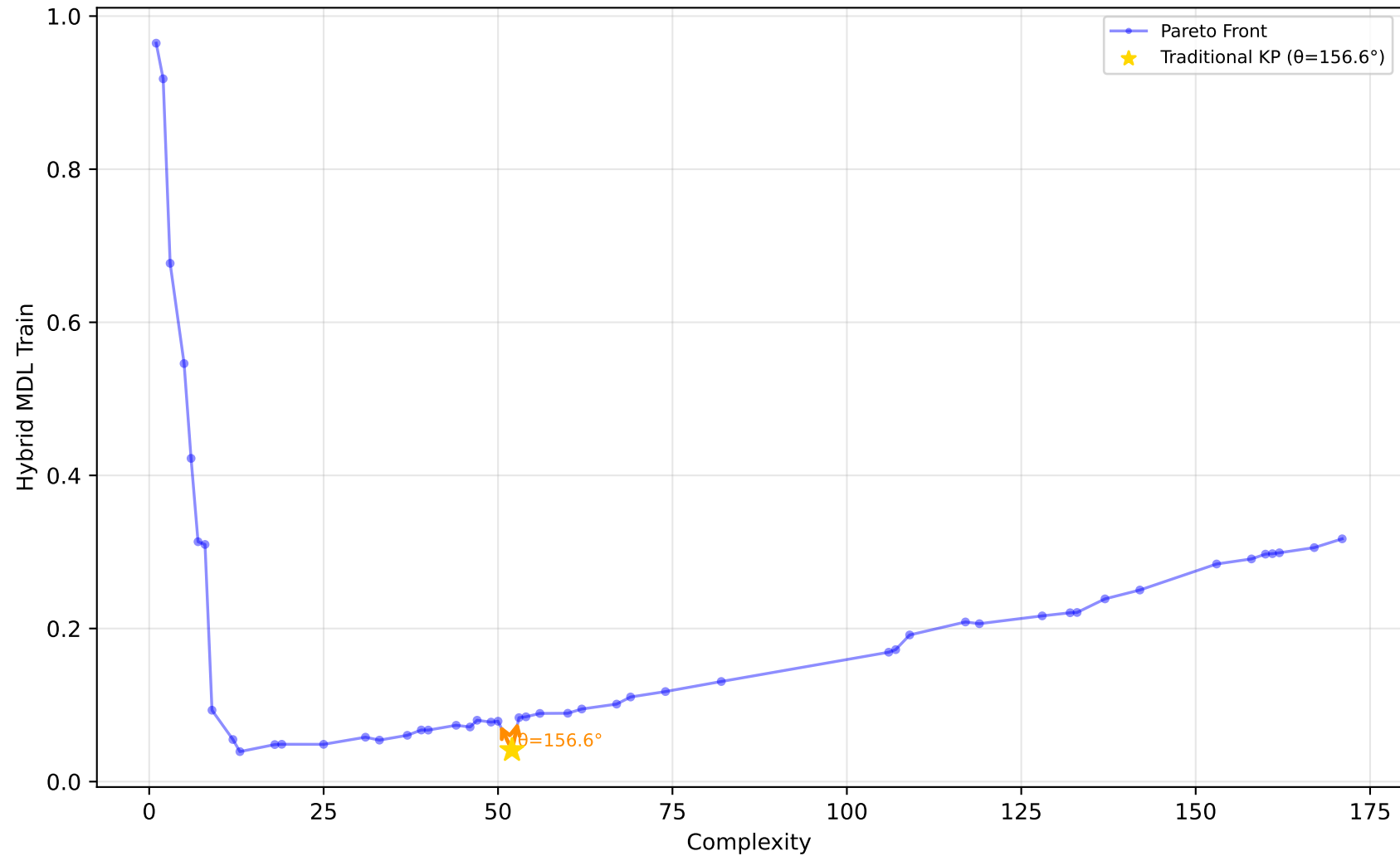
529_pollen - Run 26 - SVP - Hybrid MDL Train \lambda_1=0.10, \lambda_2=0.80, \lambda_3=0.30 | Difficulty: 1.00 | Method: hmr
