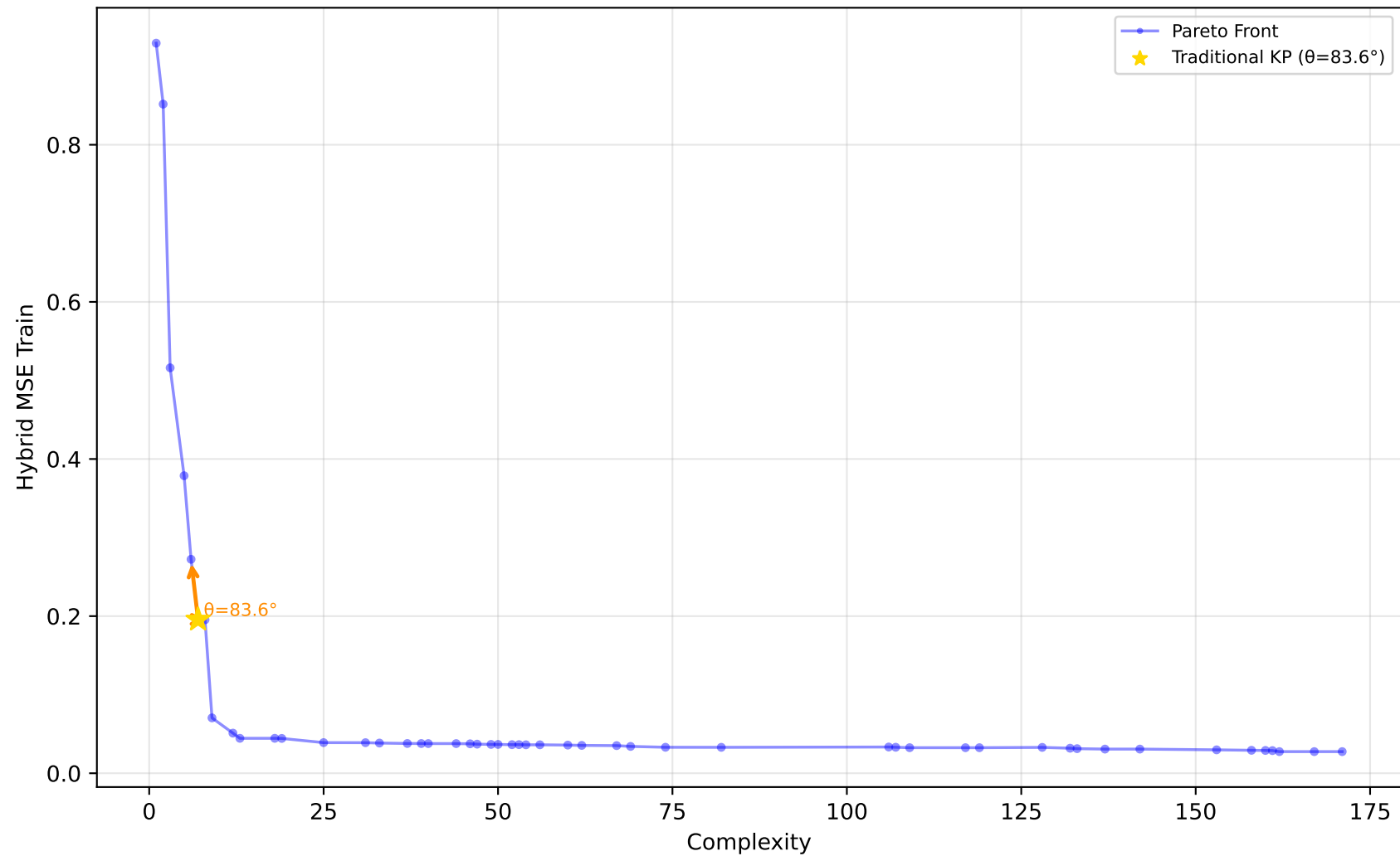
529_pollen - Run 26 - SVP - Hybrid MSE Train \lambda_1=0.10, \lambda_2=0.80, \lambda_3=0.30 | Difficulty: 1.00 | Method: hmr
