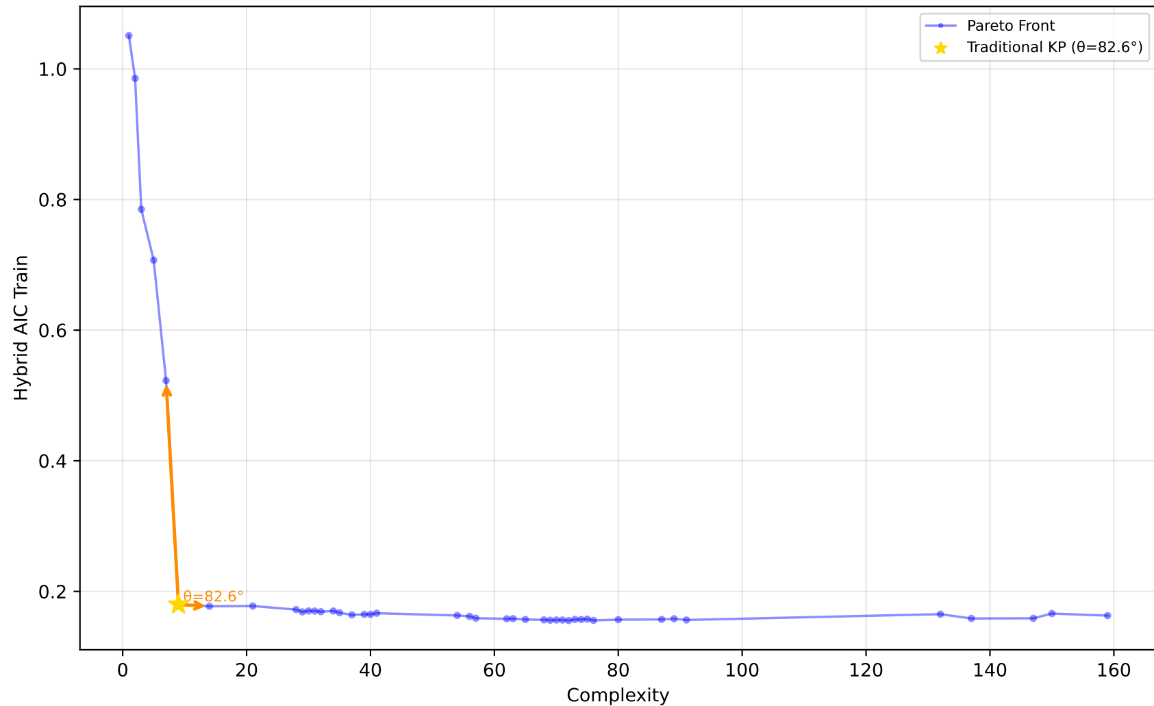
529_pollen - Run 27 - MVP - Hybrid AIC Train \lambda_1=0.90, \lambda_2=0.00, \lambda_3=0.00 | Difficulty: 1.00 | Method: hmr
