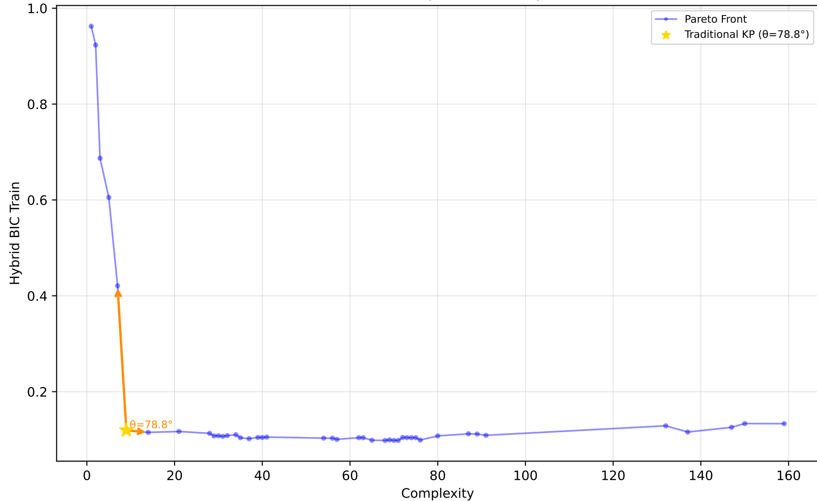
529_pollen - Run 27 - MVP - Hybrid BIC Train \lambda_1=0.00, \lambda_2=1.00, \lambda_3=0.80 | Difficulty: 1.00 | Method: hmr
