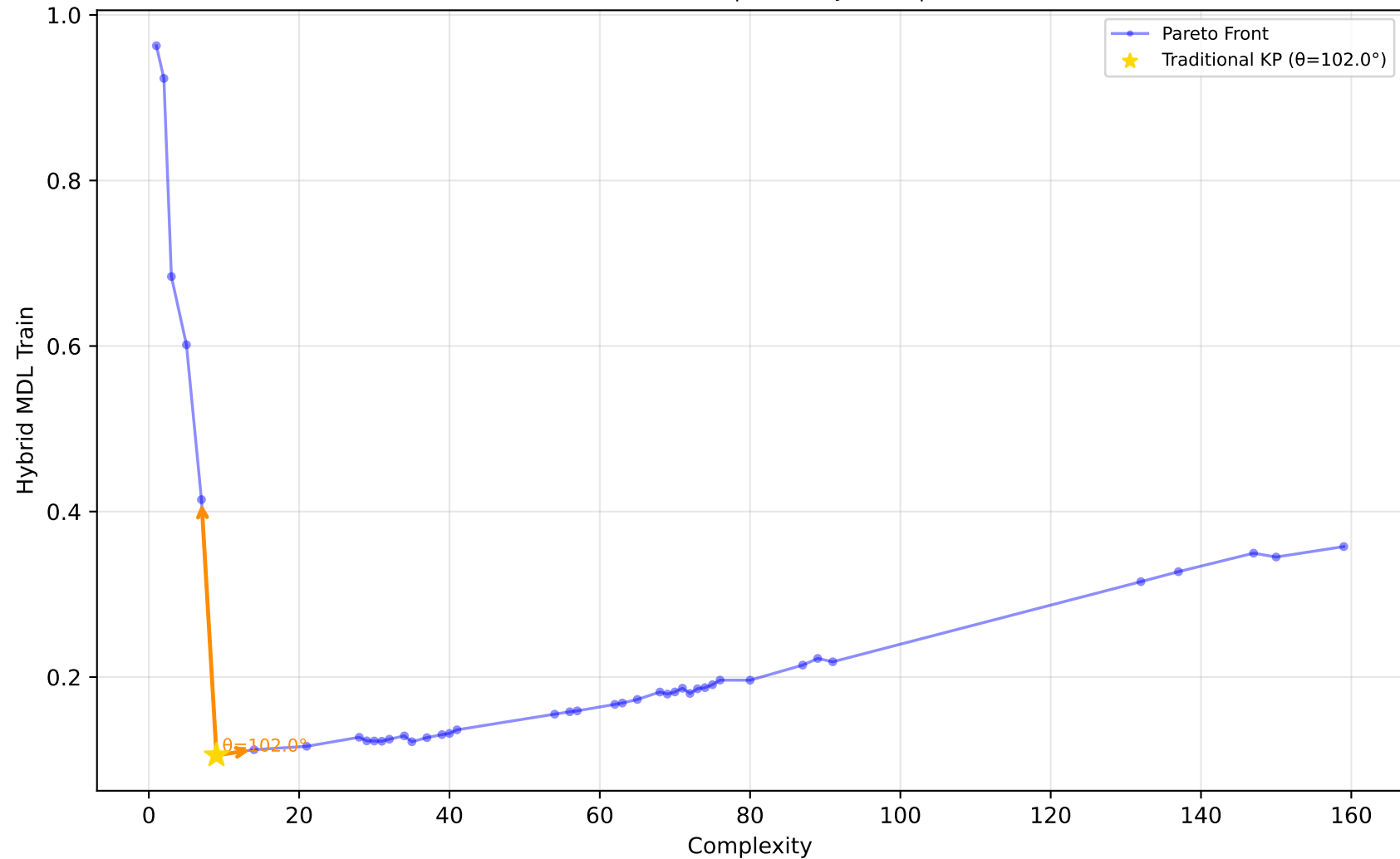
529_pollen - Run 27 - MVP - Hybrid MDL Train \lambda_1=0.00, \lambda_2=1.00, \lambda_3=0.80 | Difficulty: 1.00 | Method: hmr
